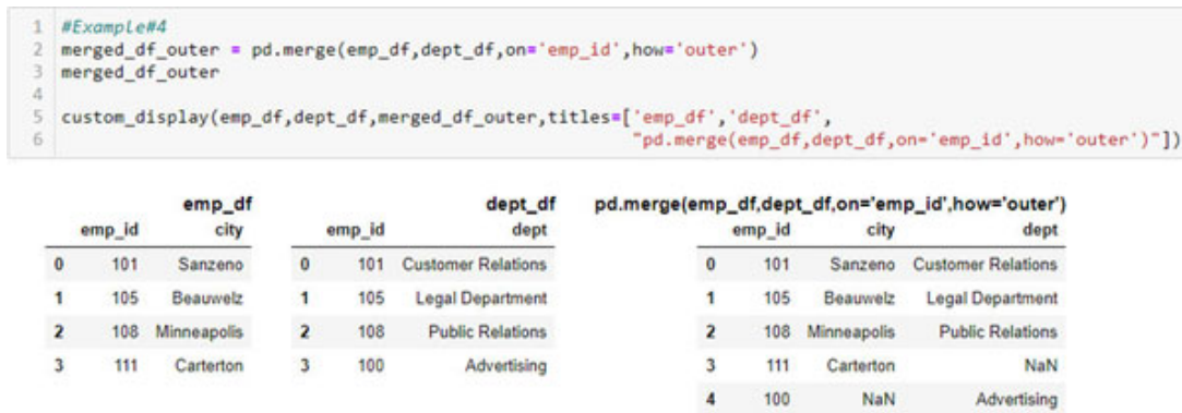
Figure 9.81: Use of merge() function with how=outer
