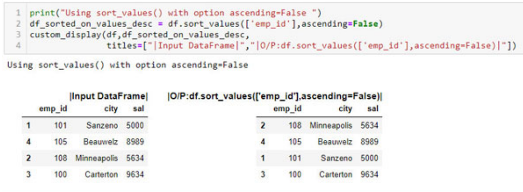
Figure 9.55: Use of sort_values() with descending order
