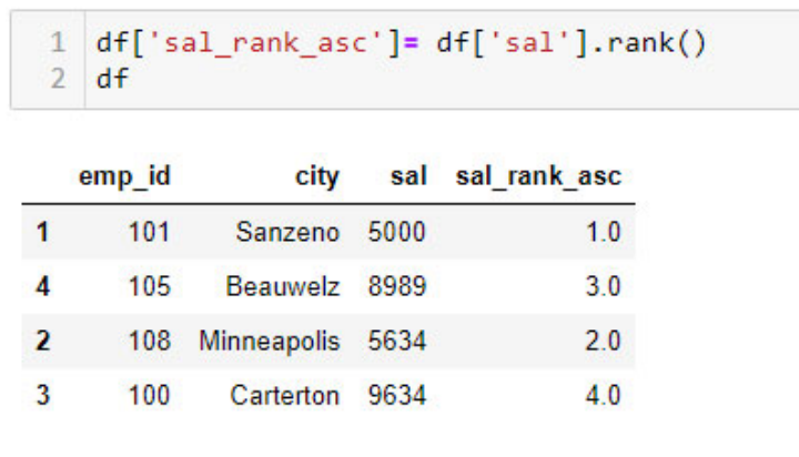
Figure 9.56: Use of rank() function
