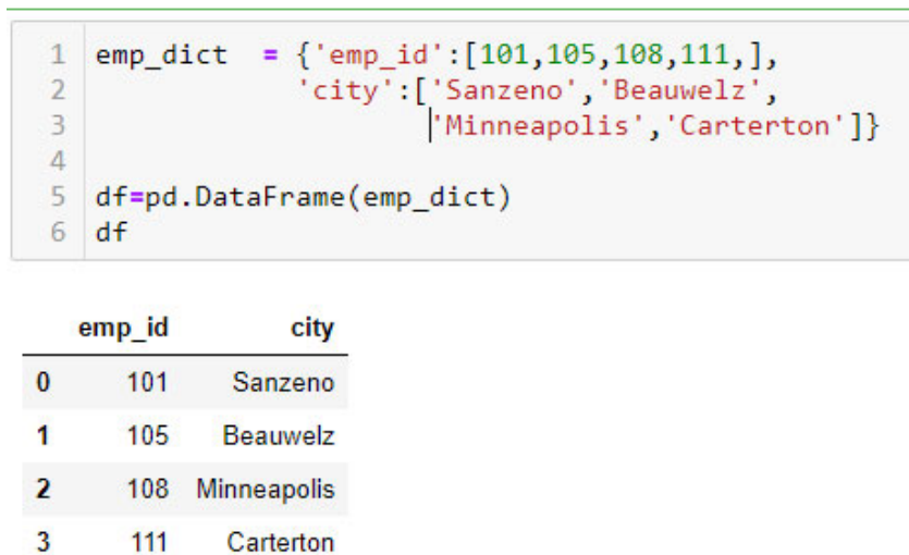
Figure 9.88: Sample dataframe
